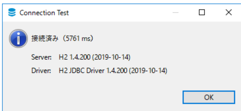
図 68. Connection Test
