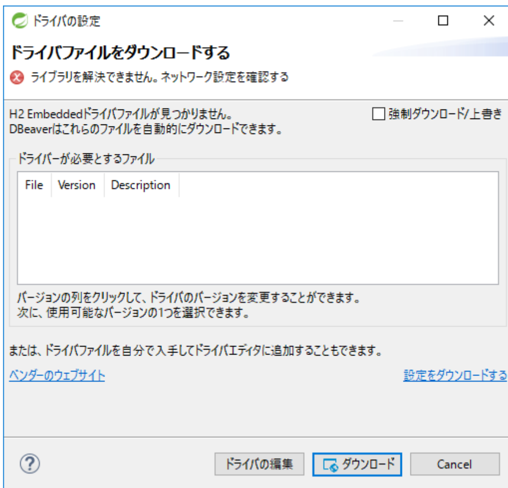
図 67. Download Driver
