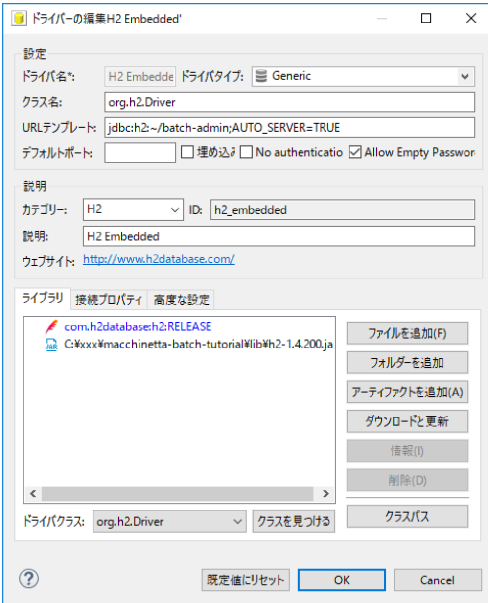
図 64. Edit Driver
