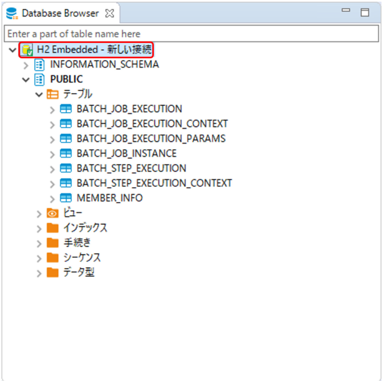
図 116. Data Source Explorer View
