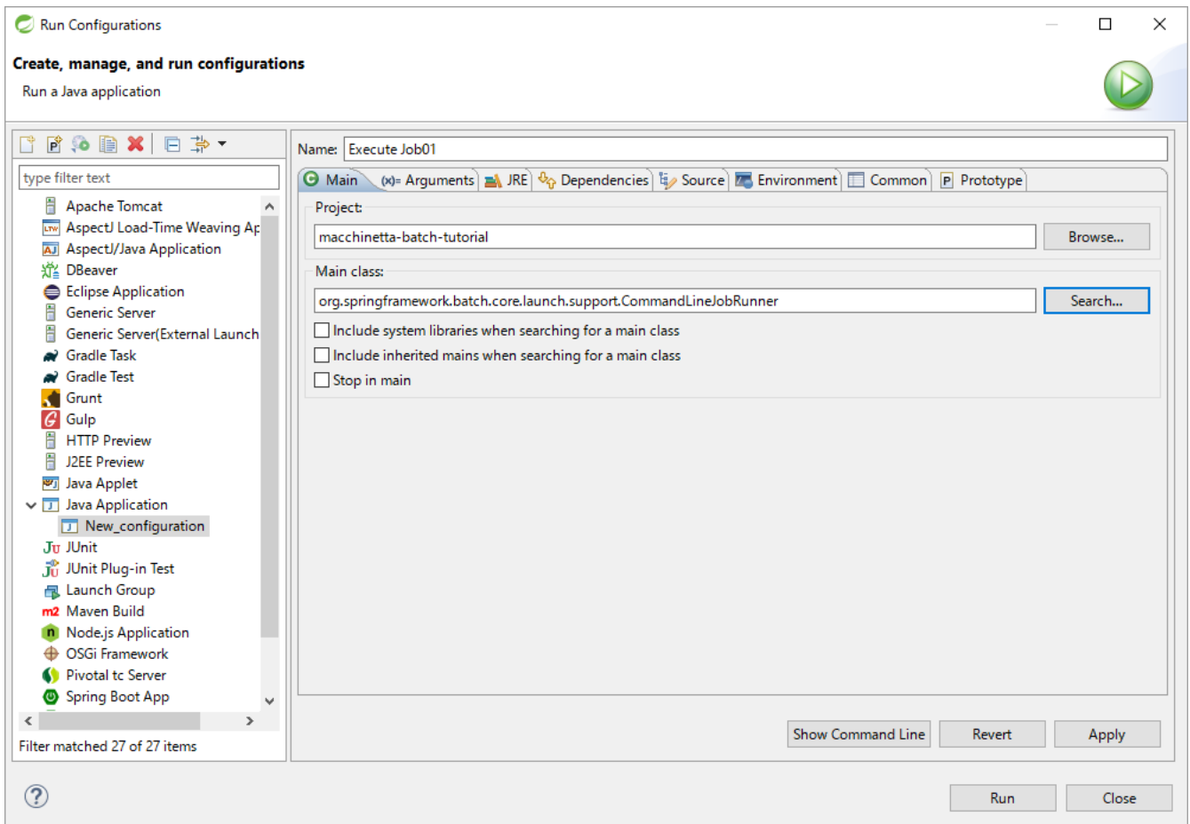
図 69. Run Configurations Main tab
