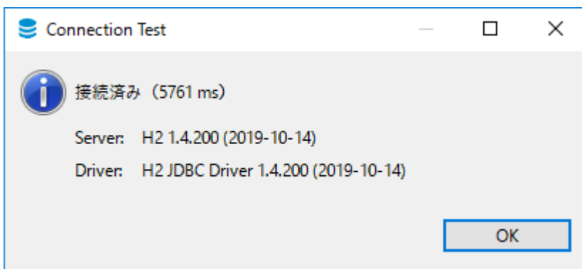
図 68. Connection Test
