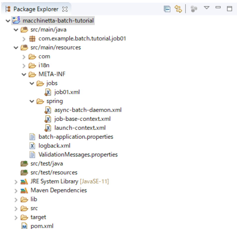
図 58. Package Explorer
