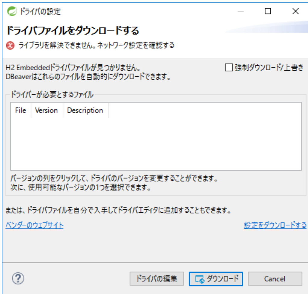
図 67. Download Driver
