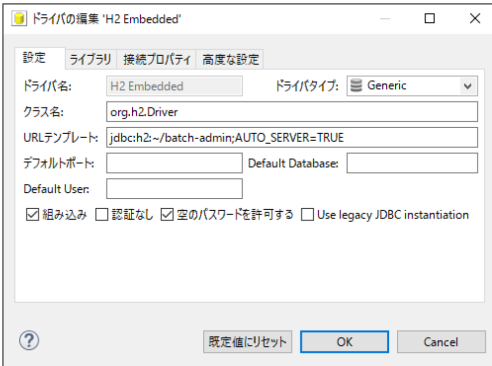
図 64. Edit Driver
