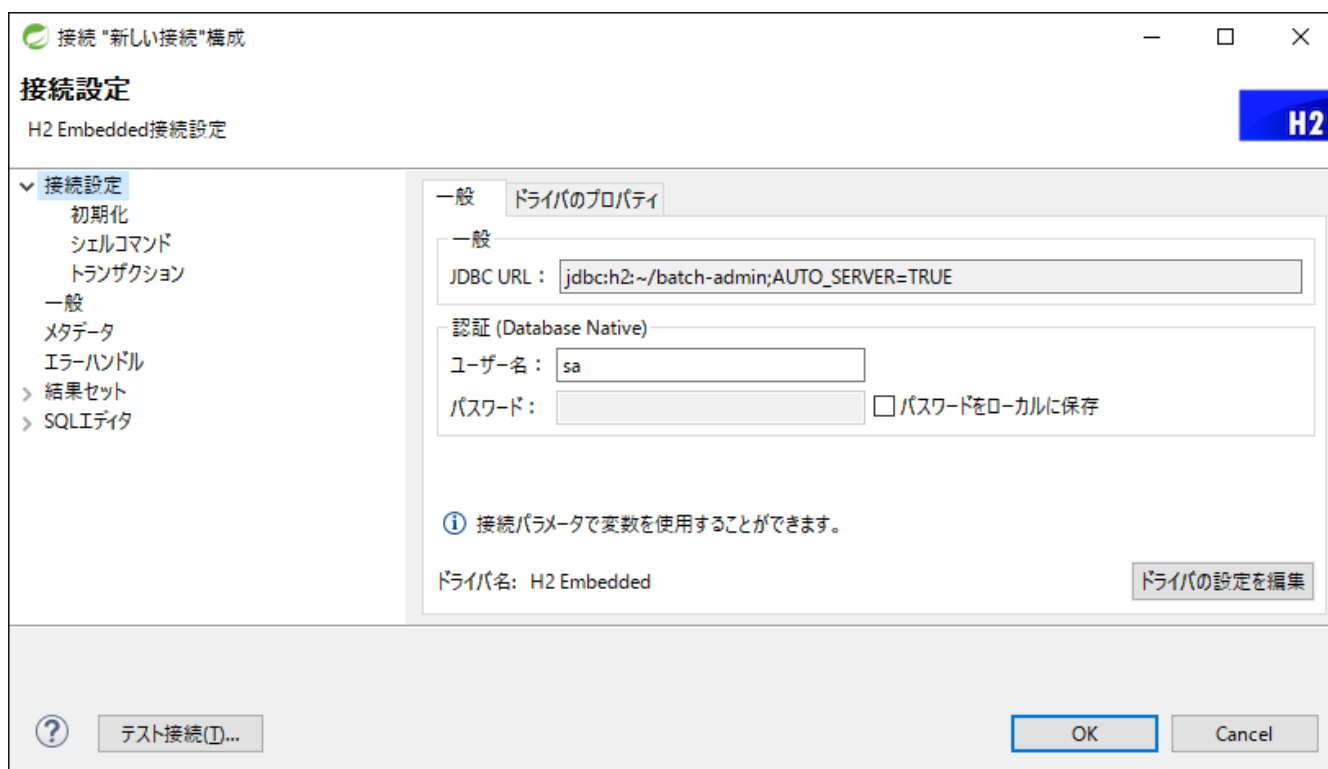
図 66. Setting Connection
