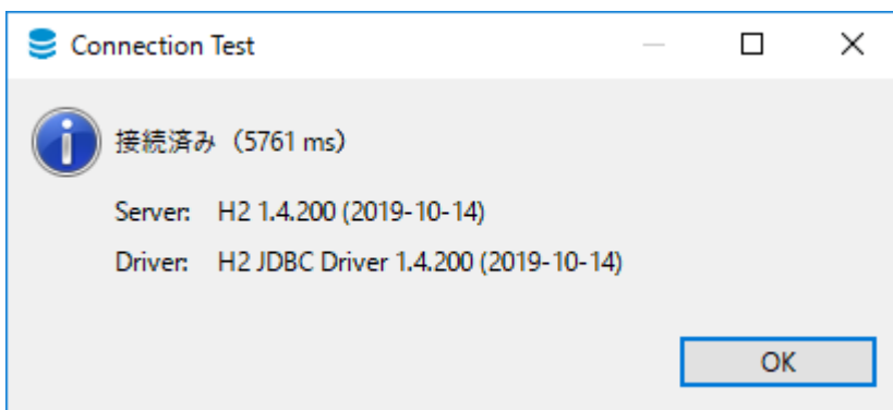
図 68. Connection Test
