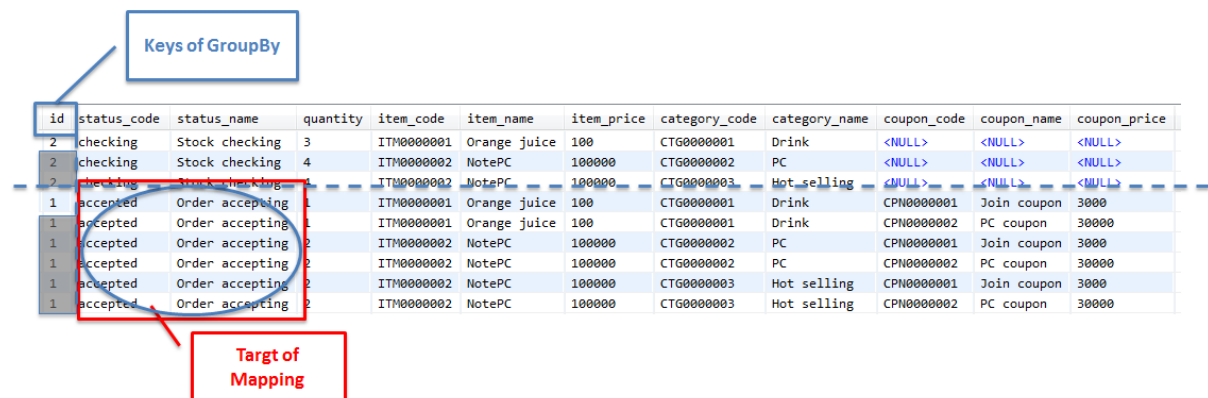
図 10 Picture - resultMap for OrderStatus
