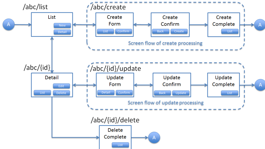
図 3 Picture - Screen flow of entity management function and assigned URL
