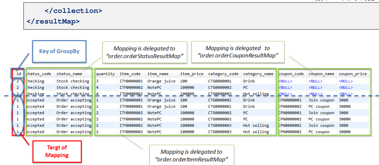
図 9 Picture - resultMap for Order
