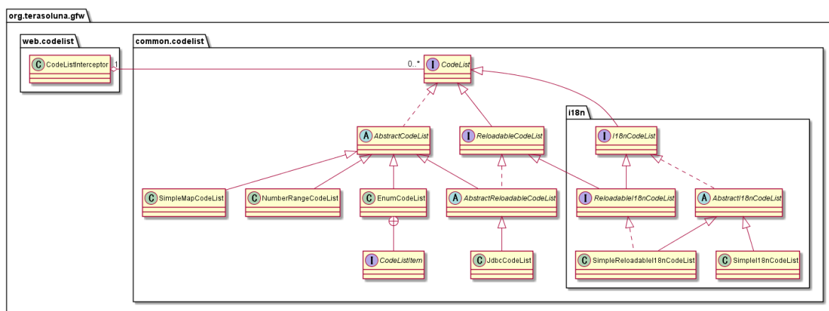
図 17 Picture - Image of codelist class diagram
