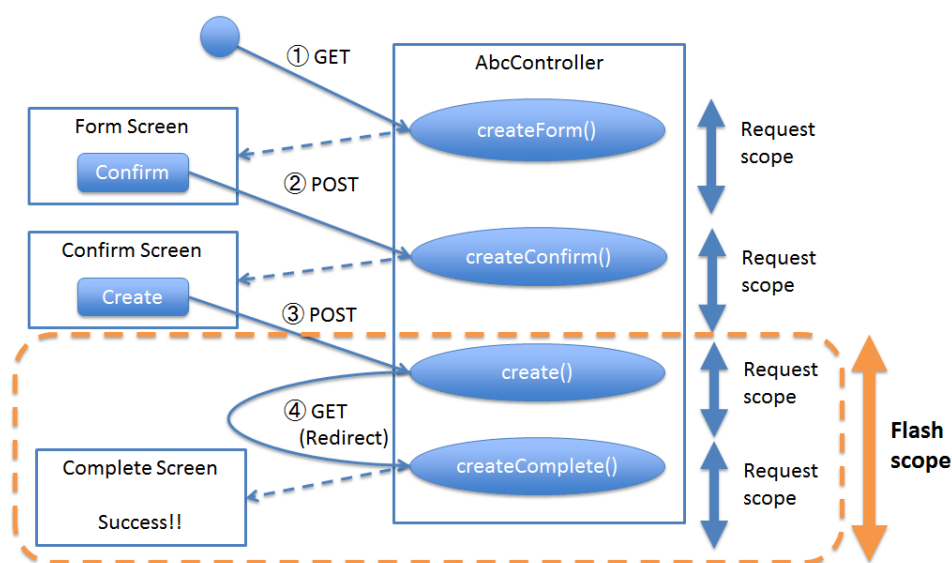
図 3.6 Picture - Survival time of flash scope
