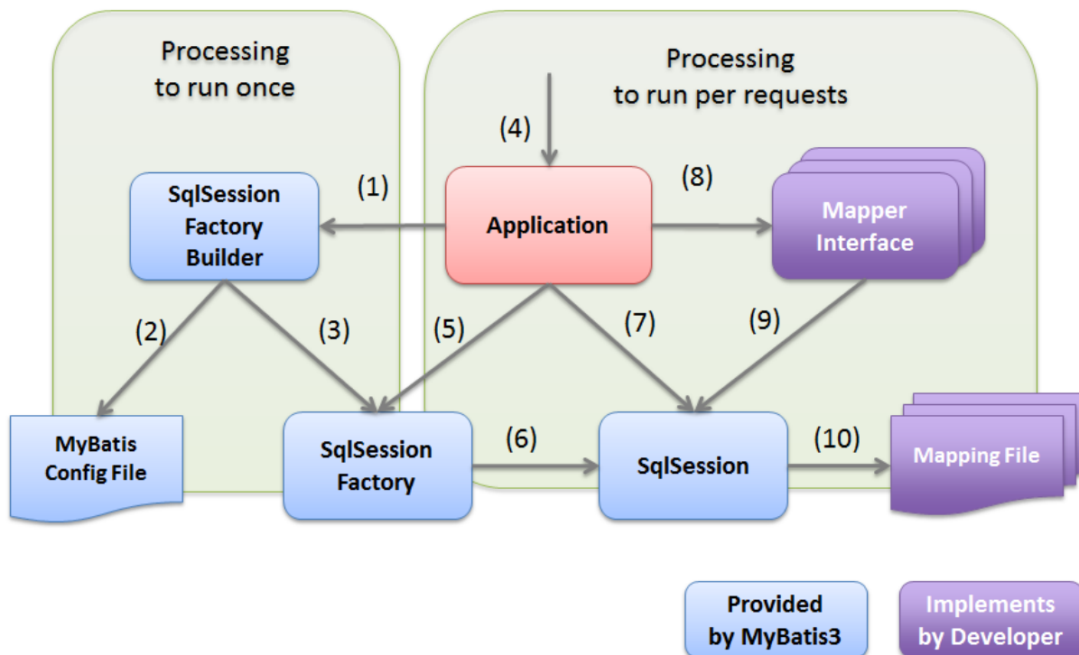
図 6.3 Picture - Relationship of MyBatis3 components
