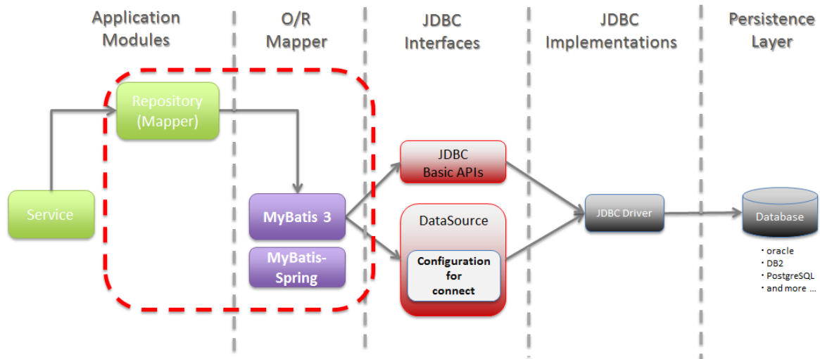
図 6.2 Picture - Scope of description
