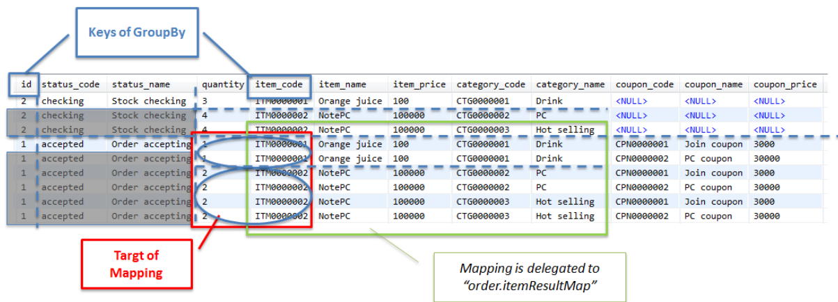
図 6.11 Picture - resultMap for OrderItem
