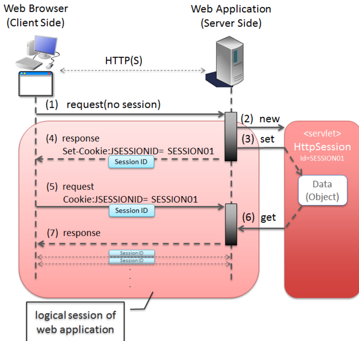
図 4.13 Picture - Establishment of logical session
