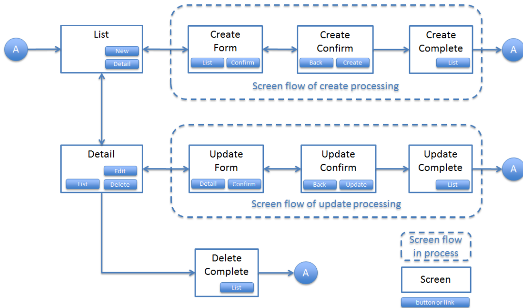
図 3.2 Picture - Screen flow of entity management function
