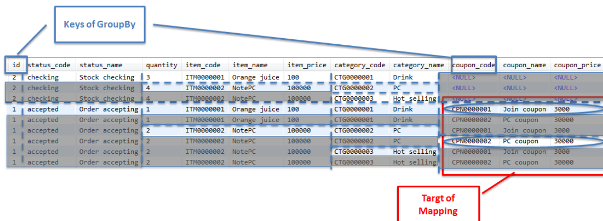
図 6.15 Picture - resultMap for Coupon
