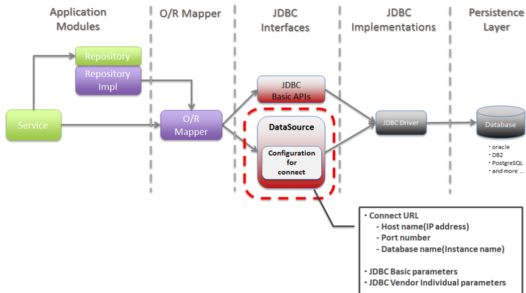
図 6.1 Picture - About JDBC DataSource
