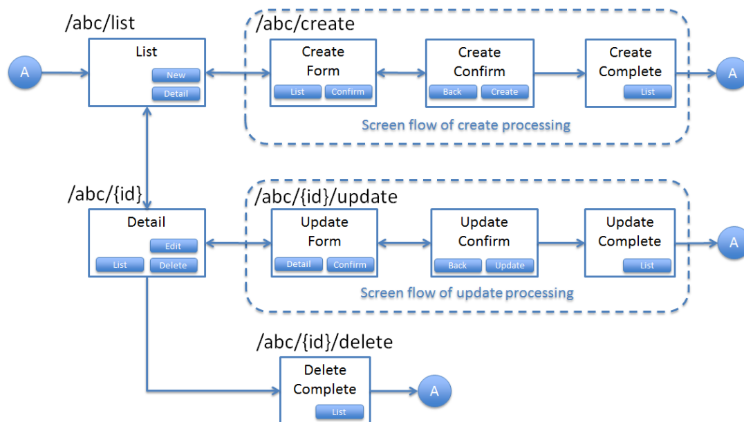
図 3.3 Picture - Screen flow of entity management function and assigned URL
