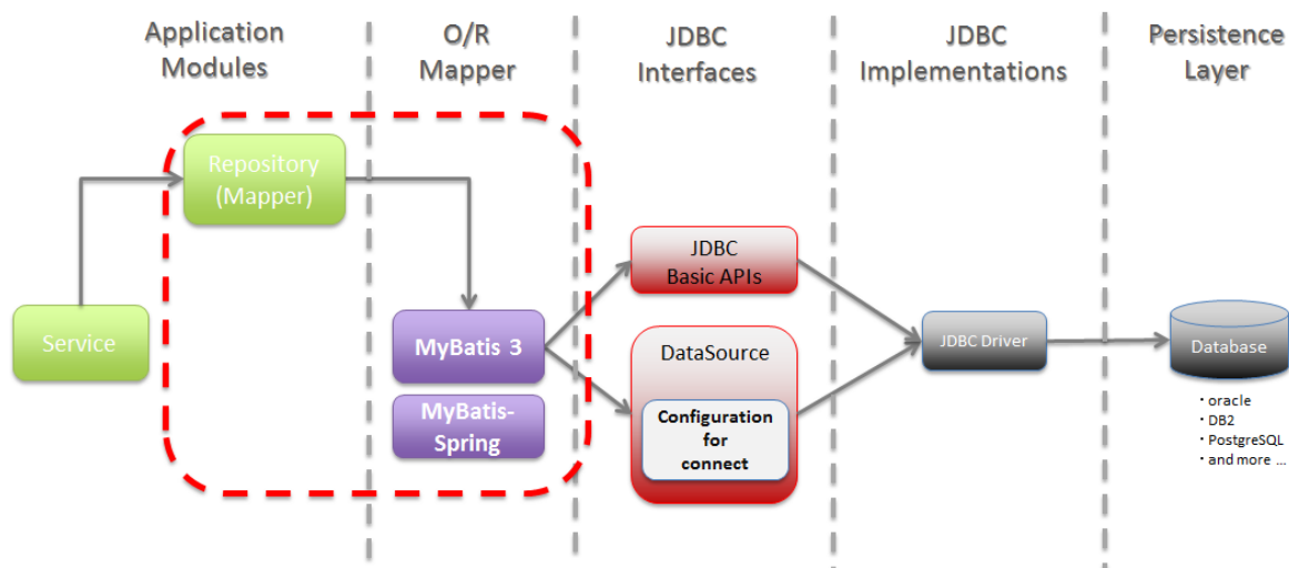
図 6.2 Picture - Scope of description
