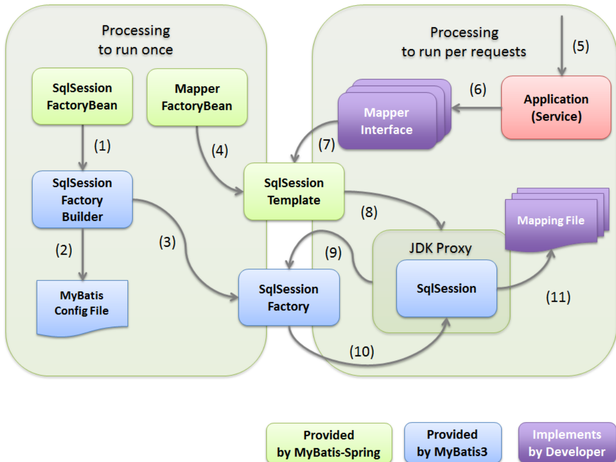
図 6.4 Picture - Relationship of MyBatis-Spring components
