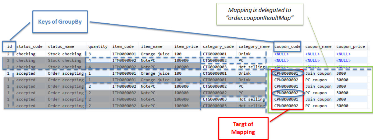
図 6.14 Picture - resultMap for OrderCoupon
