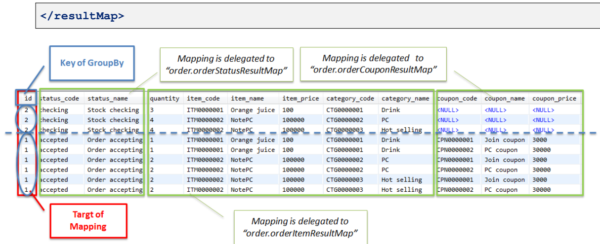
図 6.9 Picture - resultMap for Order
