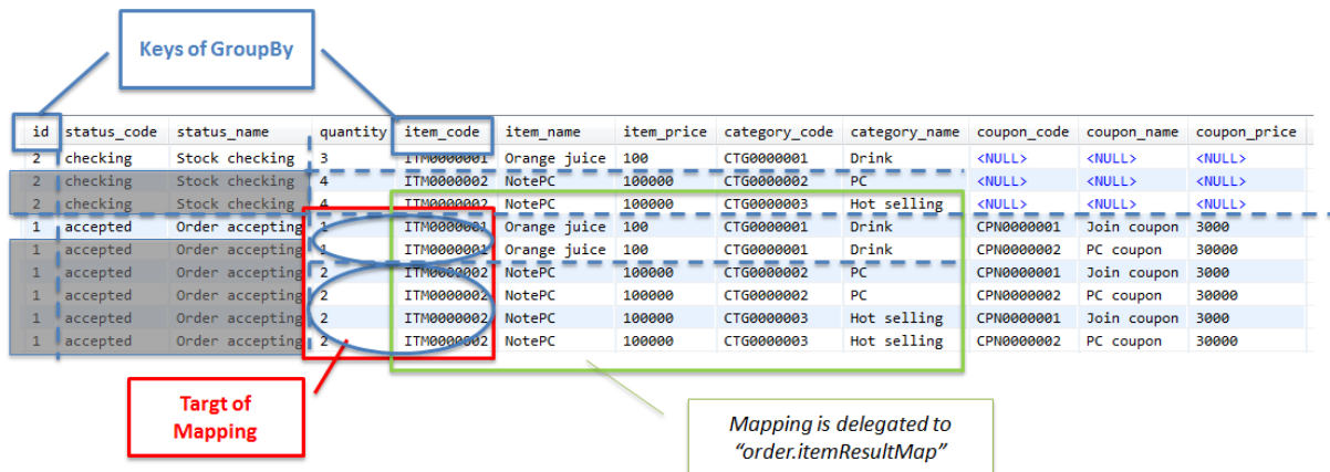
図 6.11 Picture - resultMap for OrderItem
