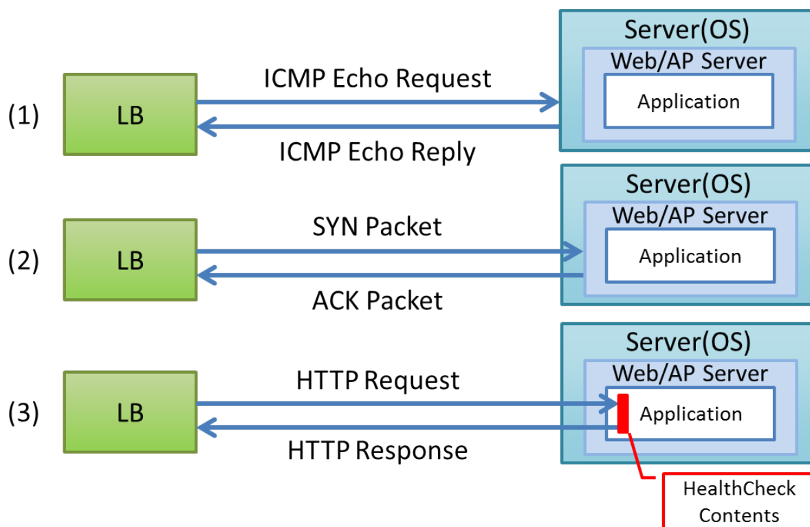
図 4.24 Picture - HealthCheck Example
