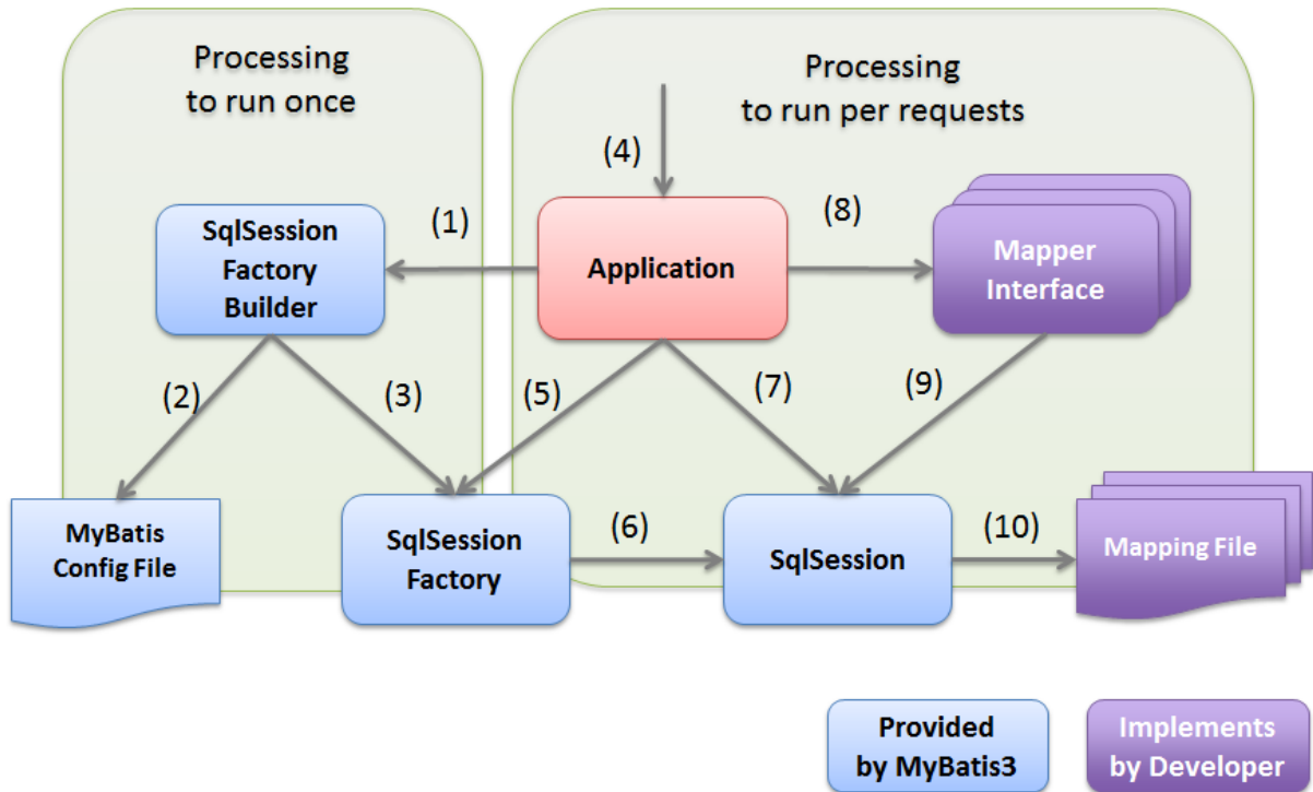
図 6.3 Picture - Relationship of MyBatis3 components
