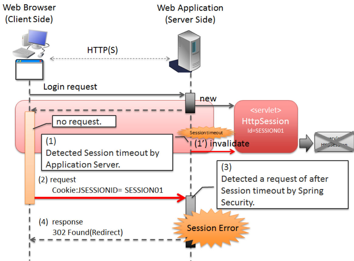
図 4.16 Picture - Detected a request of after session timeout by Spring Security
