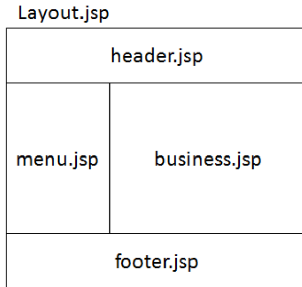
図 4.21 Picture - Image of layout.jsp
