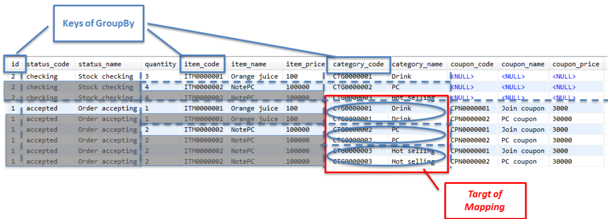
図 6.13 Picture - resultMap for Category
