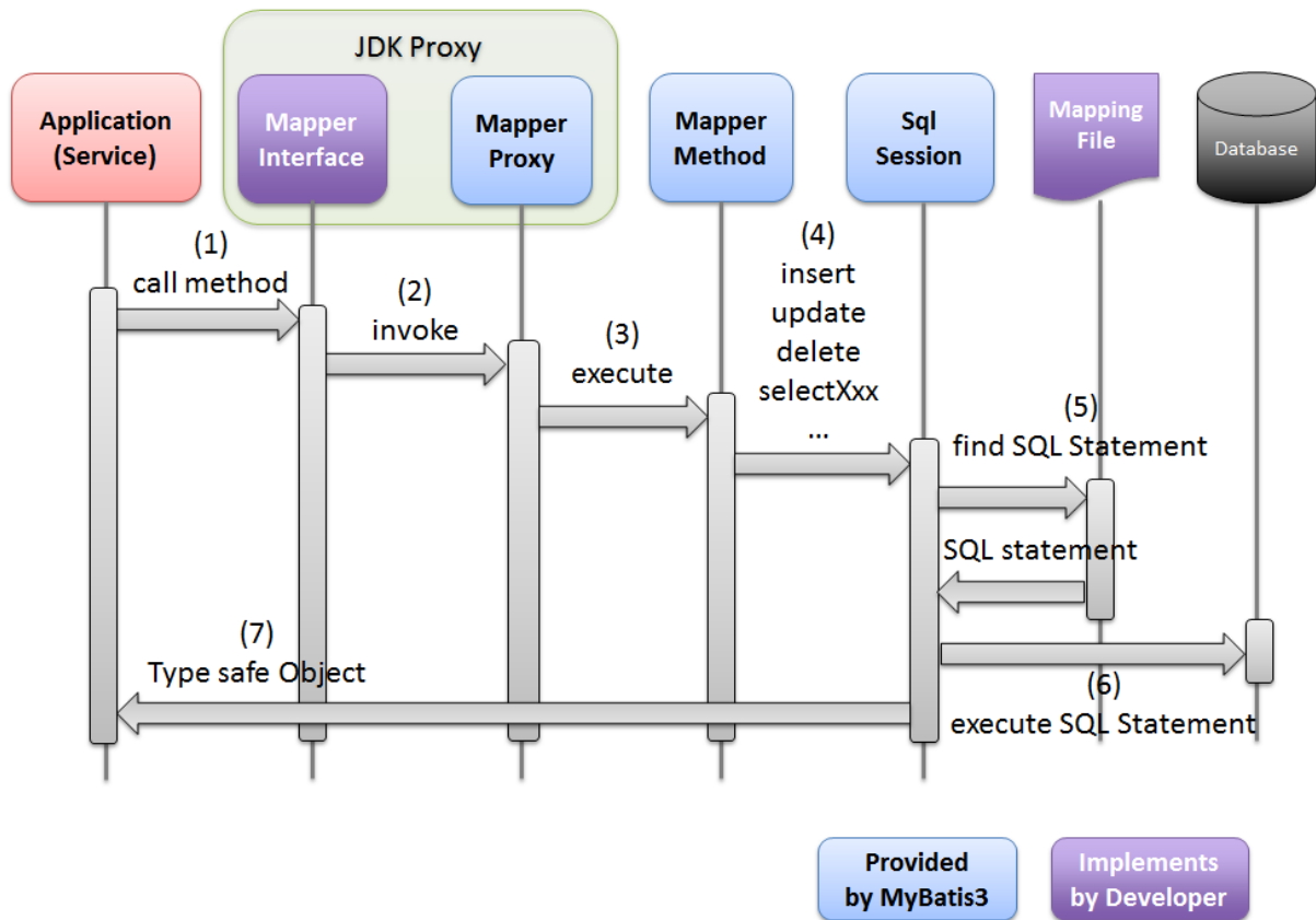
図 6.5 Picture - Mapper mechanism
