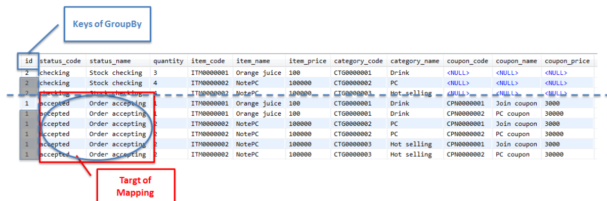
図 6.10 Picture - resultMap for OrderStatus
