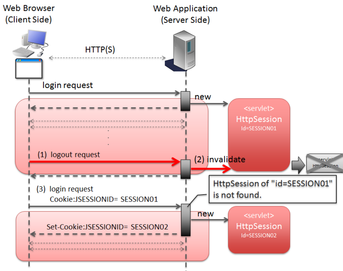
図 4.14 Picture - Invalidate session by processing of Web Application
