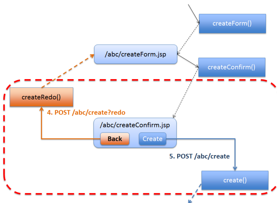
図 3.5 Picture - Multiple button in the HTML form
