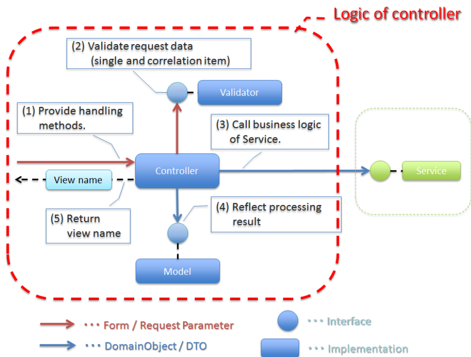
図 3.1 Picture - Logic of controller
