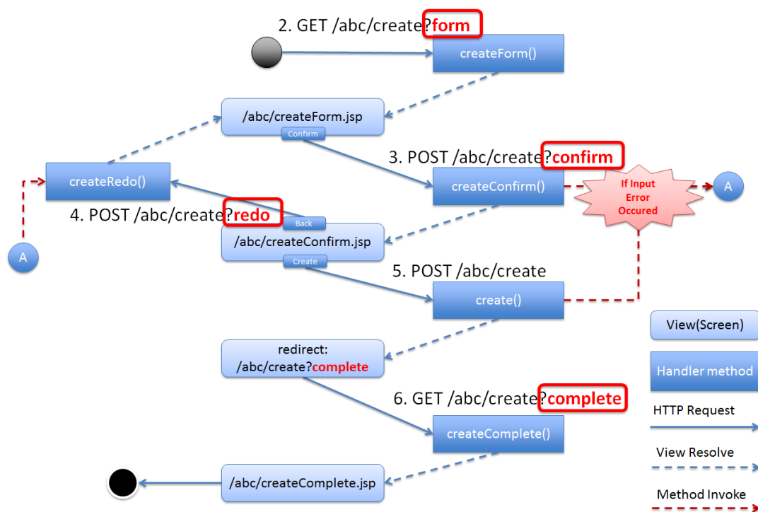
図 3.4 Picture - Request flow of entity create processing
