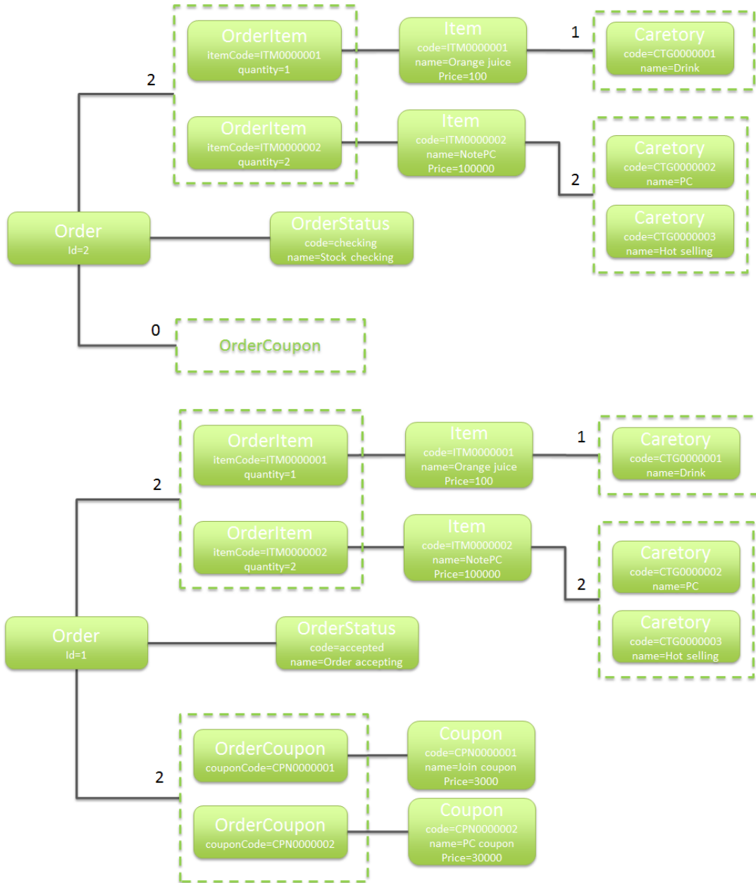
図 6.16 Picture - Mapped object diagram
