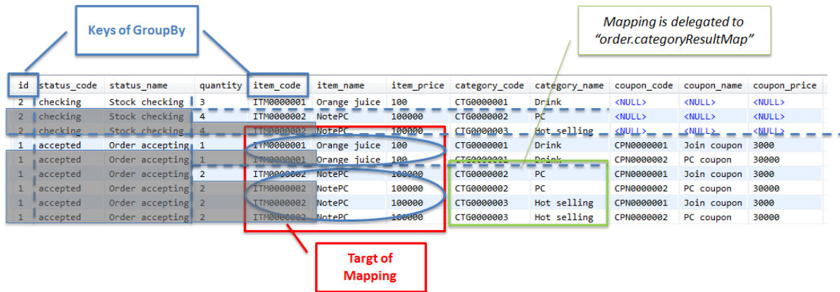
図 6.12 Picture - ResultMap for Item
