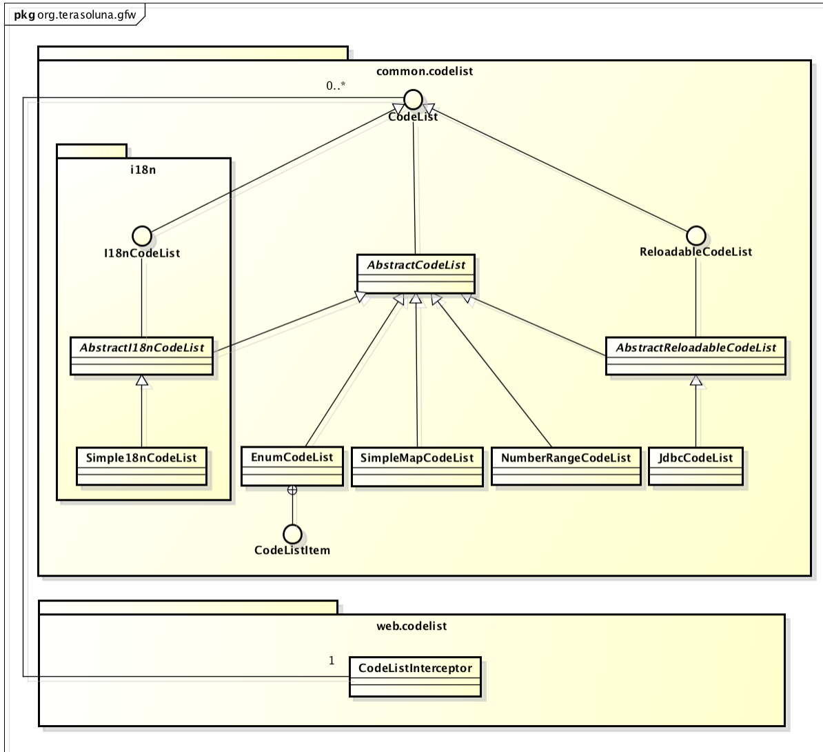
図 4.17 Picture - Image of codelist class diagram
