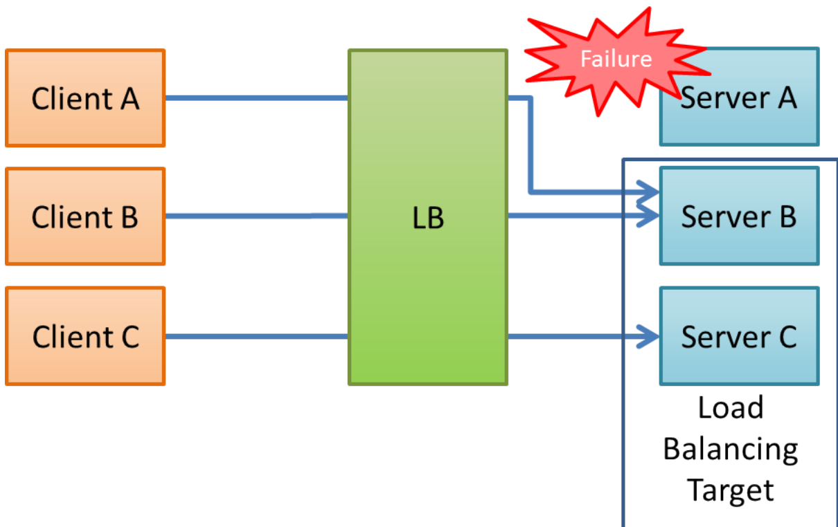
図 4.23 Picture - About Fallback
