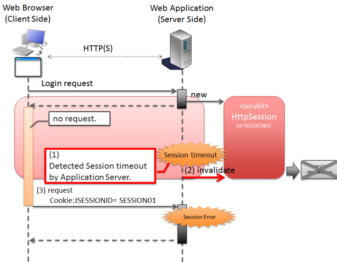
図 4.15 Picture - Invalidate session by Application Server
