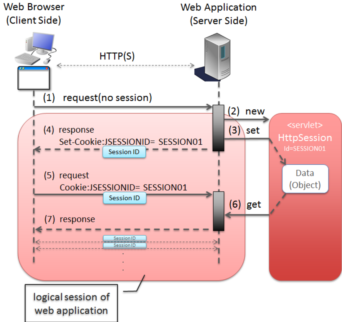
図 4.13 Picture - Establishment of logical session
